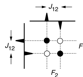
Schematic view of the cross-peak multiplet from a COSY spectrum. The circles are supposed to indicate the two-dimensional double absorption lineshape illustrated below; filled circles represent positive intensity, open represent negative intensity.
