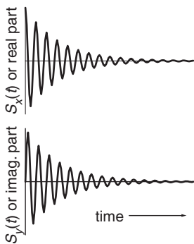
Fig. 4.4 Illustration of a typical FID, showing the real and imaginary parts of the signal; both decay over time.
